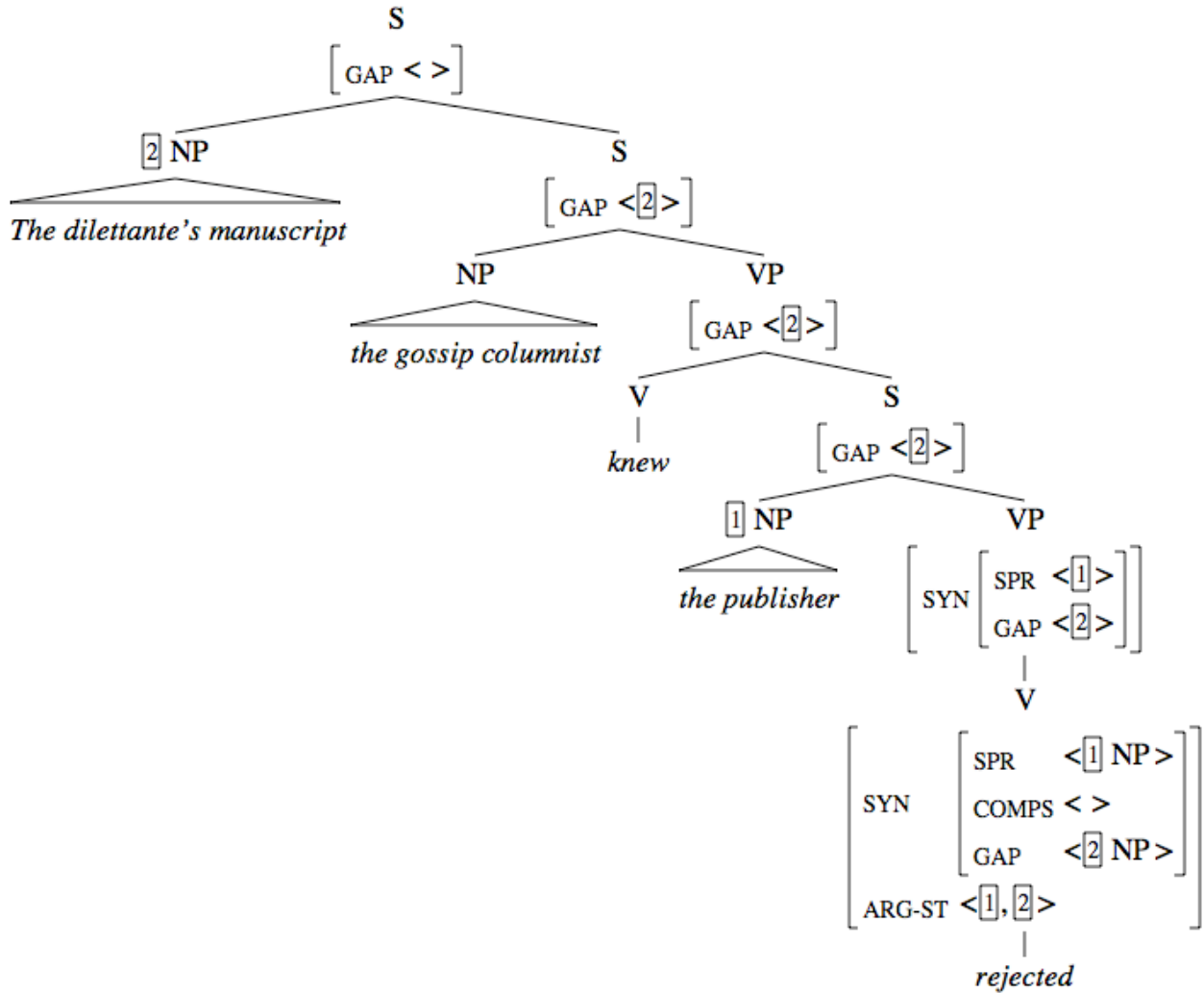
Figure 1. Schematized HPSG representation of sentence (13b). ARG-ST : argument structure list. COMPS : complements list (for the object arguments). SPR : specifier list (for the subject argument). GAP : gap list (for missing arguments).
